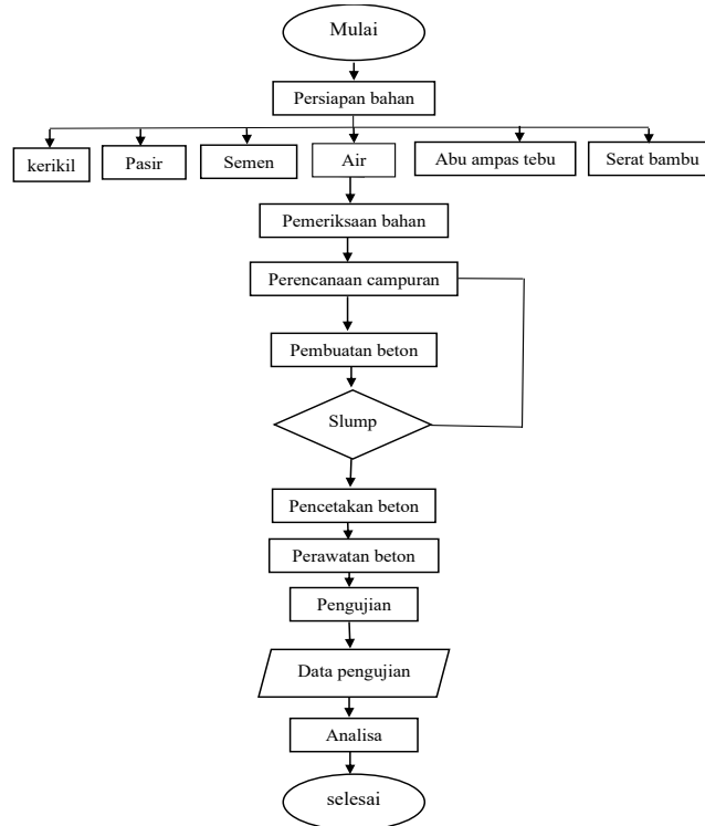
Gambar 2 Flowchart Penelitian
