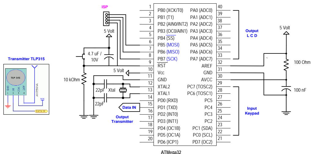
Gambar 2. Skema diagram sistem remote control
