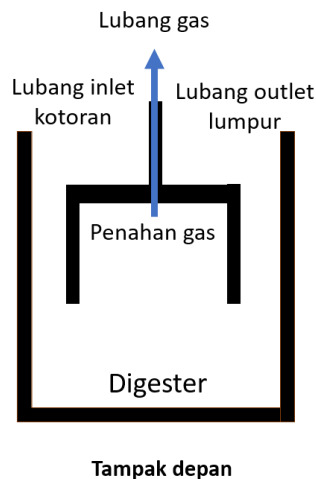
Gambar 1 Sketsa biogas concrete compact reactor
